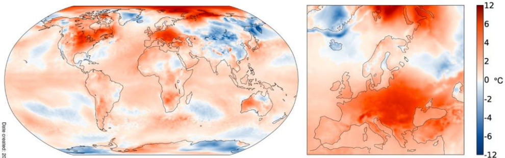
(Data: ERA5. Reference period: 1991-2020. Credit: C3S/ECMWF)
